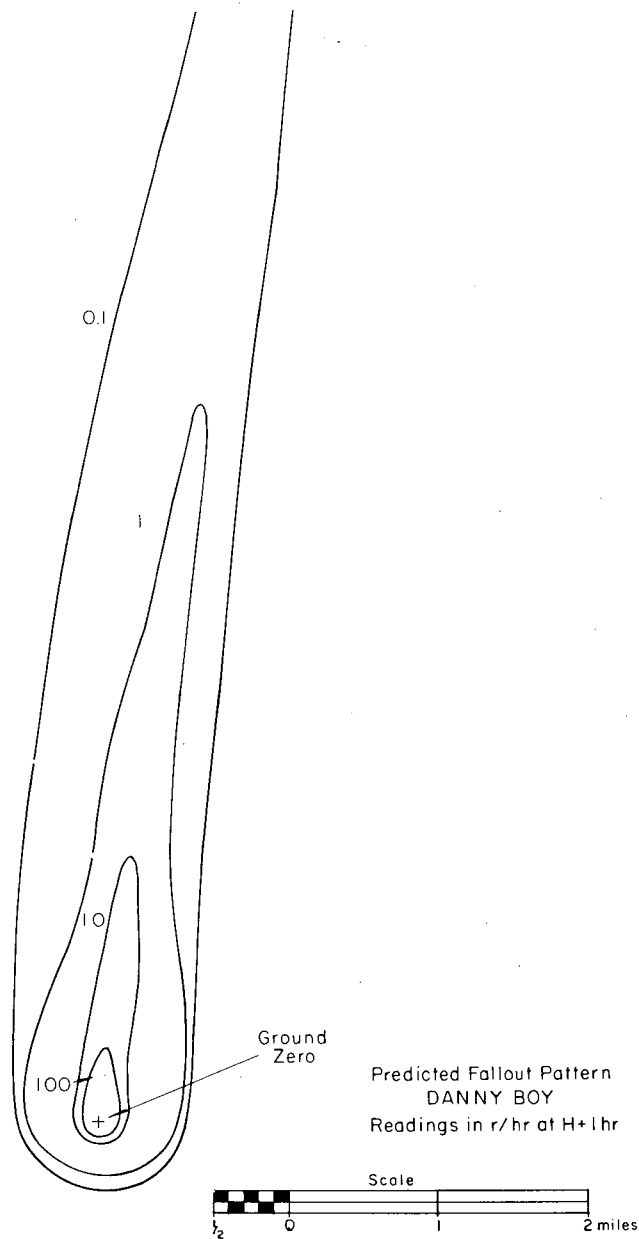
Fig. 2. Predicted fallout pattern.
